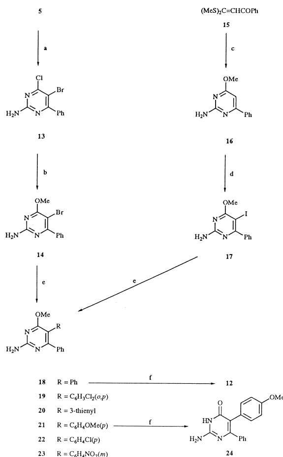
Scheme 2. Reagents: (a) \text{POCl}_3 , reflux; (b) NaOMe, MeOH; (c) guanidinium sulphate, NaOMe, reflux; (d) N -iodosuccinimide, \text{CHCl}_3 ; (e) Suzuki reactions (see Table 1); (f) 10 M-HCl, MeOH, reflux.
