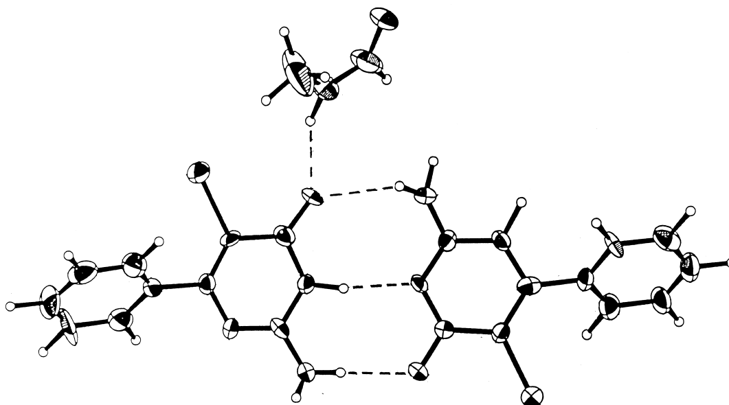
Figure 1. Hydrogen bonding between 2-amino-5-bromo-6-phenylpyrimidin-4(3 H )-one and 2-amino-5-bromo-6-phenylpyrimidin-4(1 H )-one in the crystal structure of the N -methylformamide solvate of bropirimine 5 (from ref 6). The 4(3 H )-one tautomer is shown (left), the 4(1 H )-one tautomer (right) and the molecule of N -methylformamide (above).
