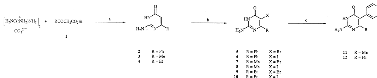
Scheme 1. Reagents: (a) EtOH reflux; (b) Br 2 in AcOH (X = Br), or I 2 in CHCl 3 –aq. NaOH (X = I); (c) Suzuki cross-coupling (see Table 1).
