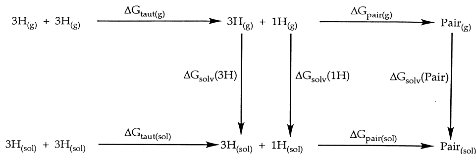
Figure 2. Free energy cycle used to calculate thermodynamic quantities. The quantities are \Delta G_{\text{taut}} , free energy of tautomerism ( 3H to 1H ); \Delta G_{\text{solv}} , free energy of solvation; \Delta G_{\text{pair}} , free energy of hydrogen-bonded pair formation.
