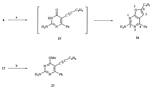
Scheme 3. Reagents: (a) NEt 3 , DMF, 1-hexyne, Pd(PPh 3 ) 2 Cl 2 –CuI, 50 °C; (b) NEt 3 , 1-hexyne, Pd(PPh 3 ) 2 Cl 2 –CuI, 50 °C.
